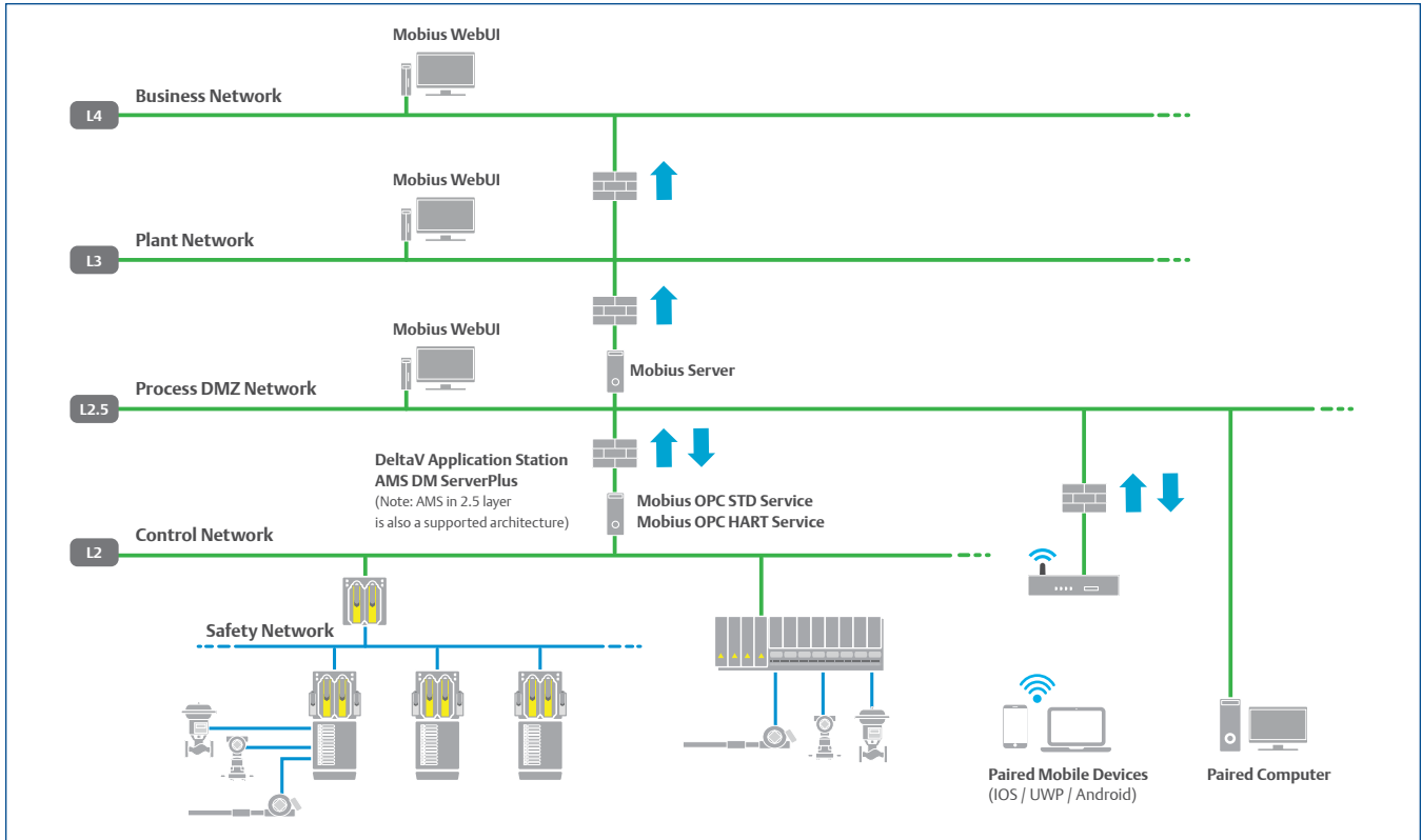
Figure 1. SIS ProofCheck Architecture.
